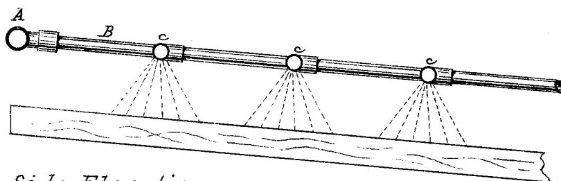
— Side Elevation — — showing water-sprays. —
