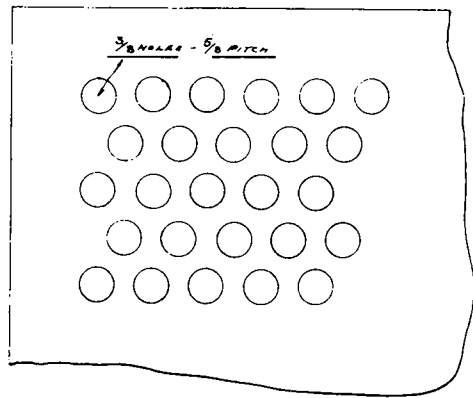
— NEW SOUTH WALES — — ASHPAN SPARK ARRESTER PLATE — — NEW ZEALAND — — ASHPAN SPARK ARRESTER PLATE —
