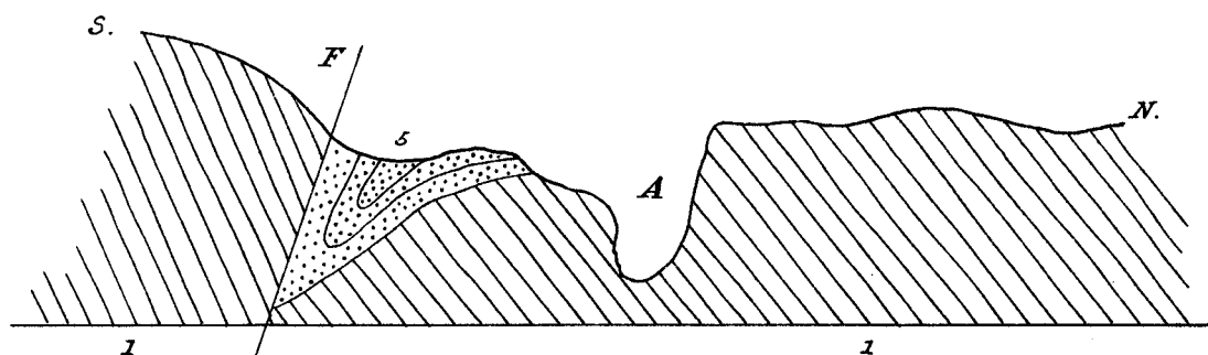
Fig 23. Sketch Section across Conroy's Gully showing the Quartz-drifts involved along line of Fault. ———
