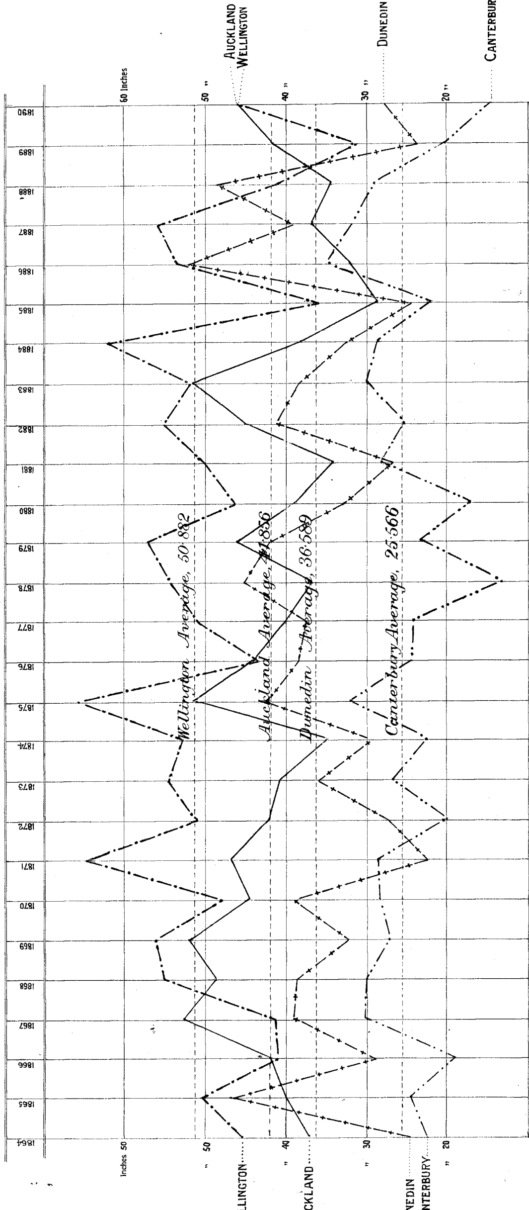
Diagram of Rain at Auckland, Wellington, Canterbury and Dunedin, 1864 to 1890.
